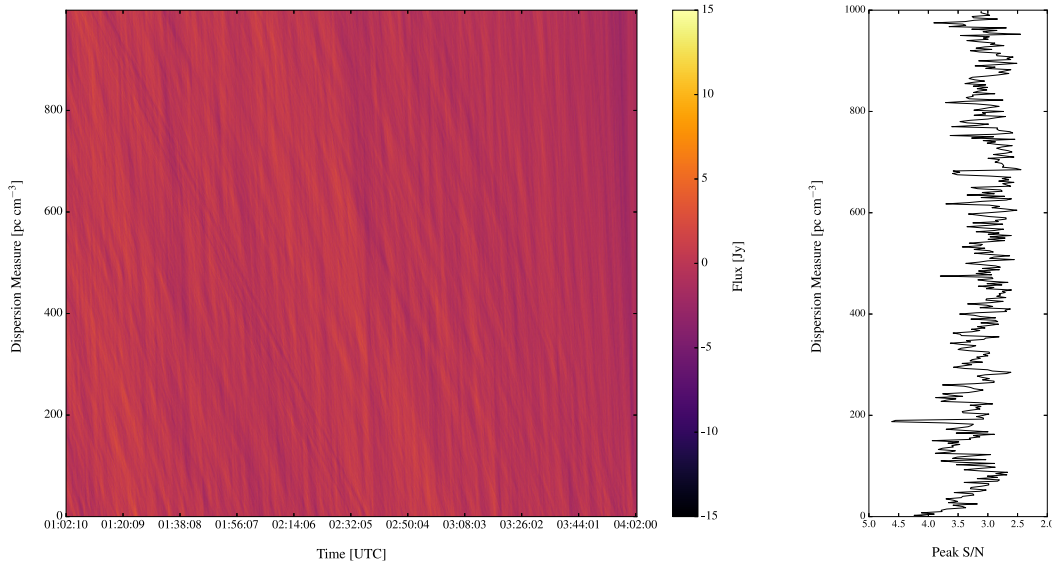
Figure 3.4: Dedispersed time series for every DM trial ranging from 0 to 1000 \text{ pc cm}^{-3} , at 2.5 \text{ pc cm}^{-3} intervals. The right panel shows the peak S/N in each dedispersed time series as a function of DM trial. No time series contains a peak S/N greater than our significance threshold. The 4.5\sigma spike just below a DM of 200 \text{ pc cm}^{-3} is 2 DM channels wide, and is due to spurious unflagged frequency channels.
