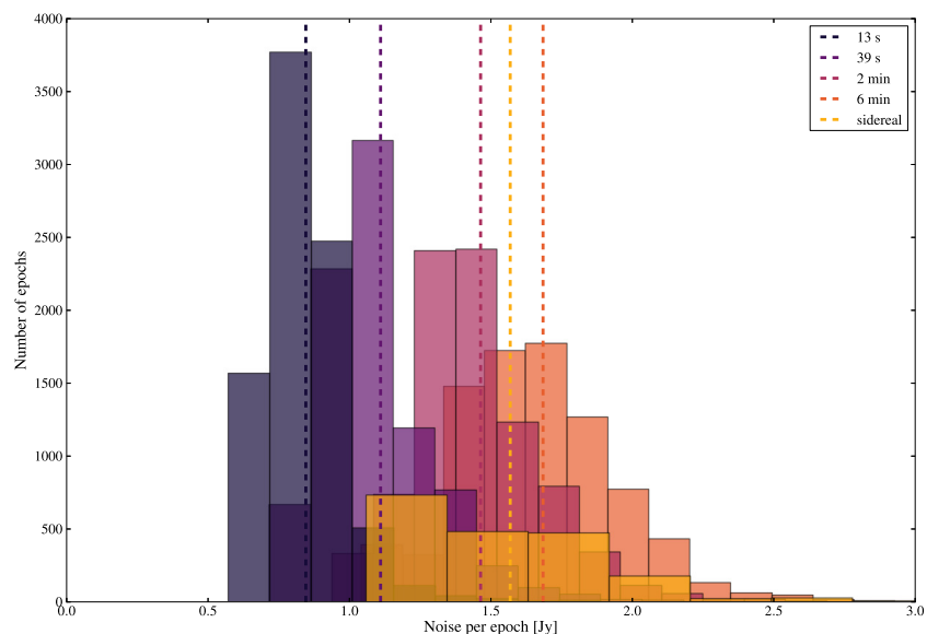
Figure 4.2: Histogram of the noise, as measured from the pixels in the 15^\circ region surrounding zenith, in each difference image epoch, for all timescales probed. The dashed lines show the mean value of the noise for each timescale.
