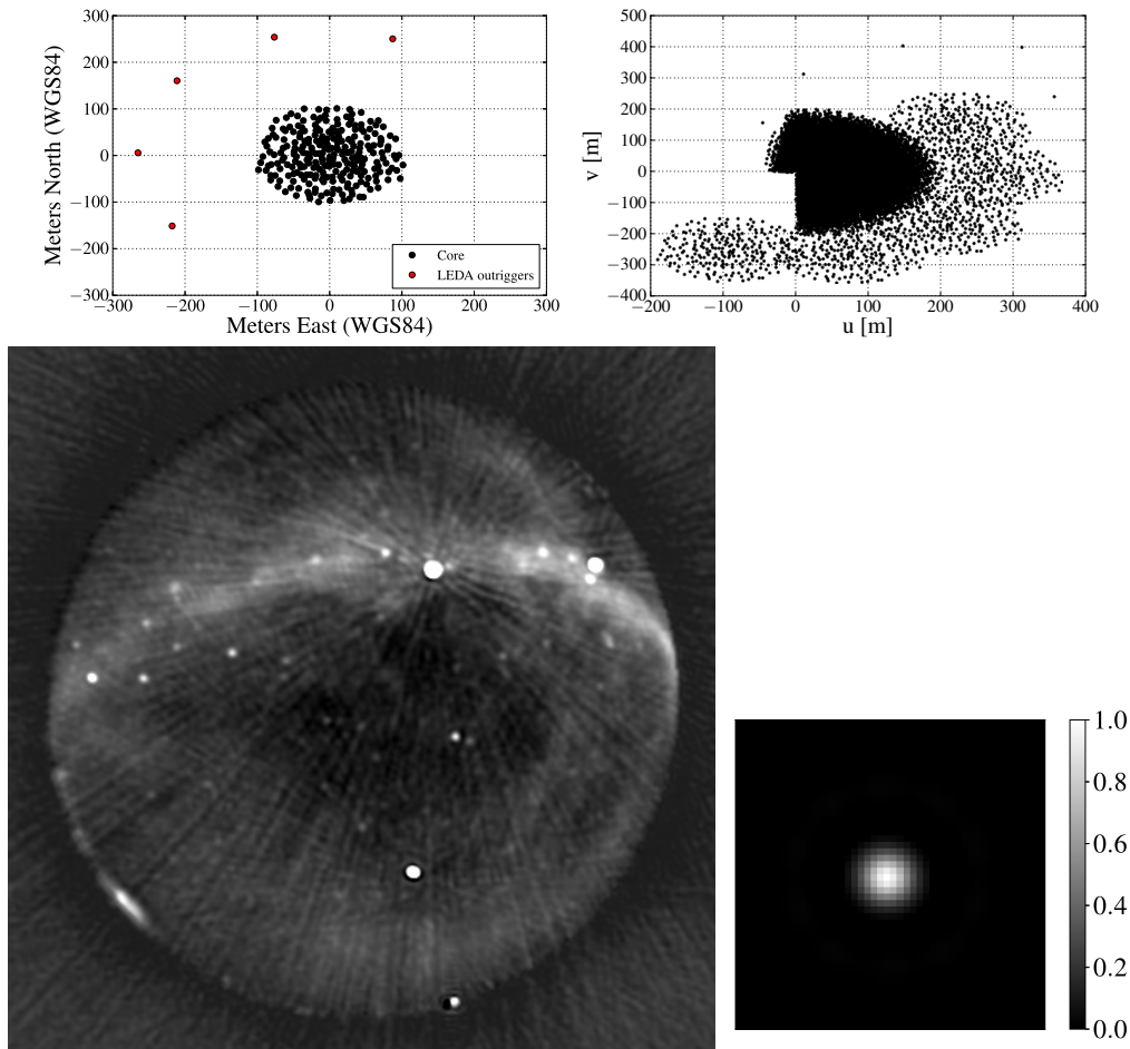
Figure 2.2: The Stage I OVRO-LWA. Map of antenna locations in the core (top left), the corresponding uv coverage (top right), the point spread function (PSF) using a Briggs robust weighting of 0 (bottom right), and an all-sky image from the Stage I array (bottom left).
