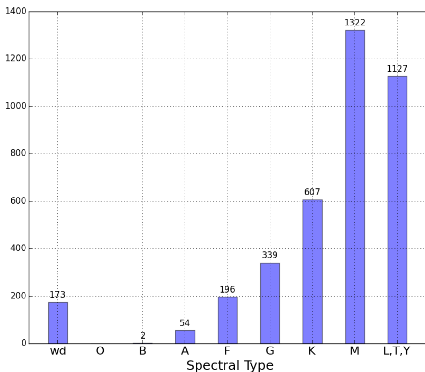
Figure 5.2: The 25-pc sample, containing 3820 objects. As expected, the sample is dominated by M dwarfs. Sources are compiled from 1) the Kirkpatrick et al. 2012 8-pc volume-limited sample; 2) the Dwarf Archives database of Kirkpatrick et al. containing all known, spectroscopically determined L, T, and Y dwarfs; 3) the Gliese Catalog of Nearby Stars, 3rd Edition; 4) the Sion et al. 2014 white dwarf 25-pc sample; and 5) the M dwarf 25-pc sample c/o Evgenya Shkolnik. We have excluded sources below -33^\circ declination.
