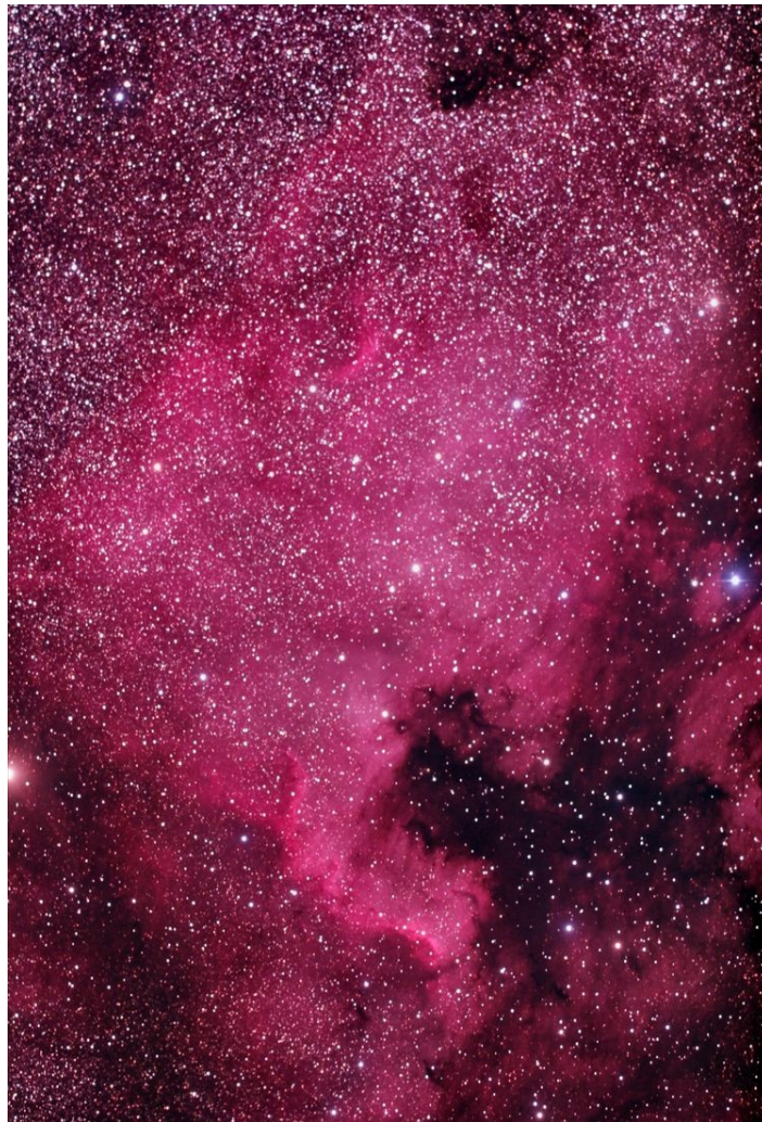
North America Nebula
